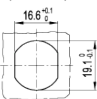
Drilling template (for stator M19)
